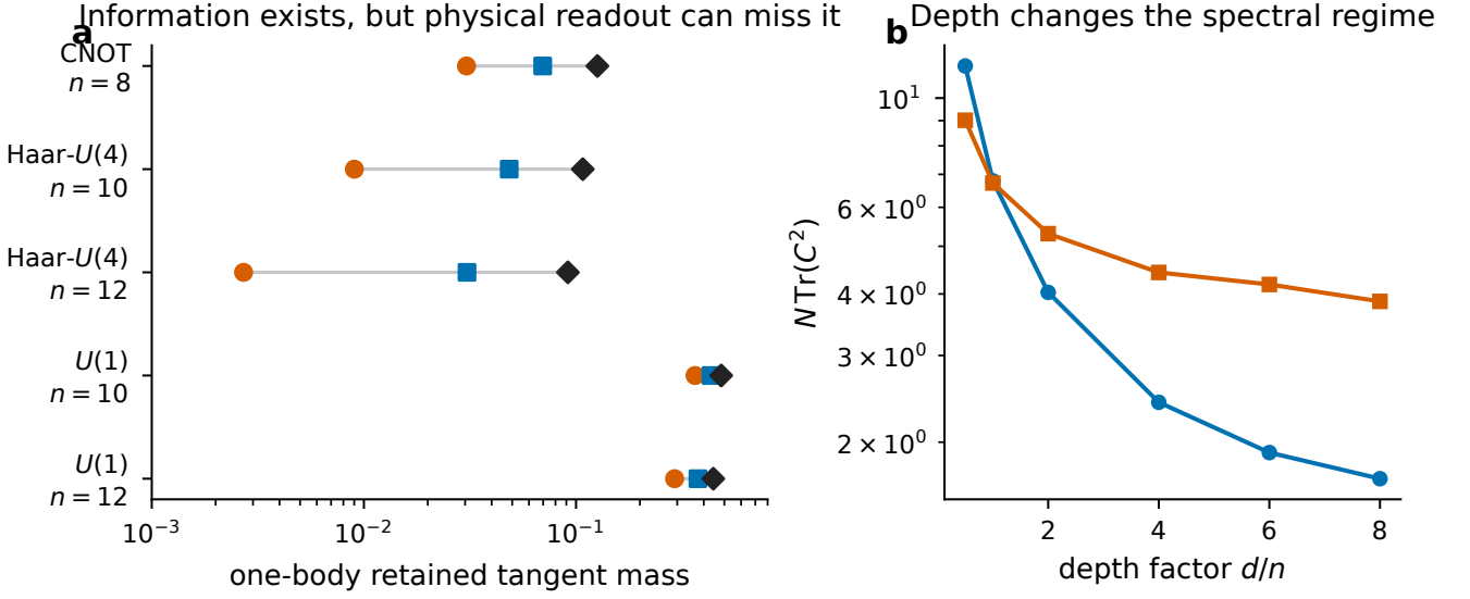
FIG. 5. Same-rank spectral comparison. Physical low-weight, cross-fitted aligned, and same-sample Ky Fan subspaces have identical rank but can retain very different tangent mass. The orientation gap is large in generic Haar- U(4) circuits and substantially smaller in the U(1) family.
