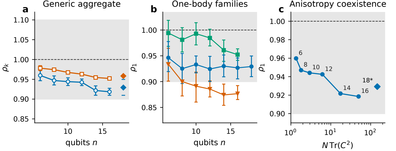
FIG. 4. Rank-normalized retention and covariance anisotropy. Family-balanced generic low-weight readouts remain close to the rank reference over the tested sizes even while N\text{Tr}(C^2) grows and d_{\text{eff}}/N decreases. Architecture-resolved data show systematic deviations, demonstrating that the family-balanced result is not a claim of literal Haar orientation.
