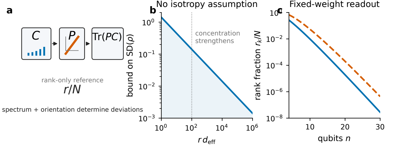
FIG. 1. Rank and orientation in measurement-accessible tangent geometry. A fixed quantum measurement induces a centered score space. A normalized tangent covariance C distributes tangent mass within that space, while a rank- r readout projector P selects the directions retained by the learner. The accessible tangent mass is R = \text{Tr}(PC) . Random relative orientation gives the rank-only reference r/N ; the spectrum of C controls the null width, while the physical orientation of P controls the observed deviation from that reference.
