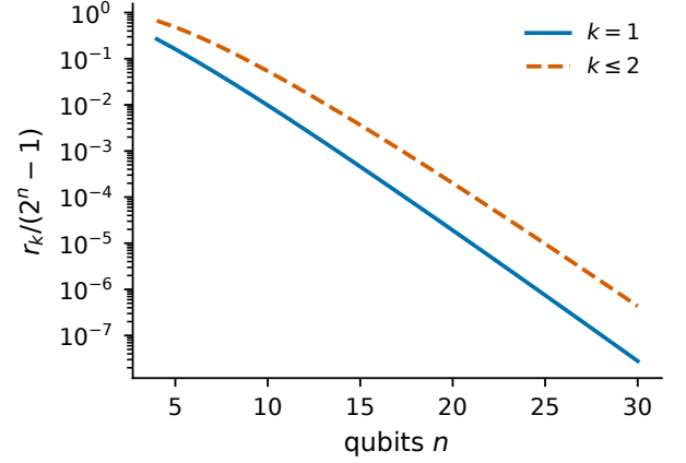
FIG. 9. Rank fractions for low-weight diagonal readouts under full computational-basis support. Polynomially growing low-weight spaces occupy an exponentially shrinking fraction of the centered record.
