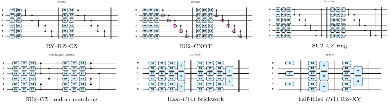
FIG. 13. Individual PennyLane circuit schematics used by the numerical campaign. Gate parameters are hidden in the drawings, while the source constructors and complete numerical profiles are archived with the code and results.
