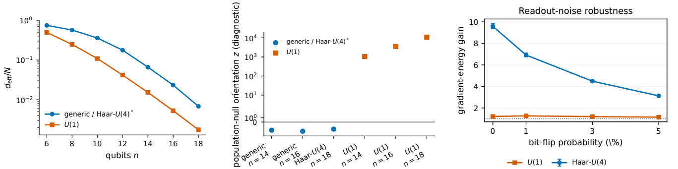
FIG. 11. Supporting diagnostics. Left: effective spectral fraction d_{\text{eff}}/N . Center: population-null orientation diagnostic for representative generic/Haar and U(1) points. Right: aligned-to-physical directional gradient-energy gain under readout bit-flip noise. The noise comparison re-estimates the aligned subspace after noise is applied and therefore does not establish robustness of a single fixed optimized observable.
