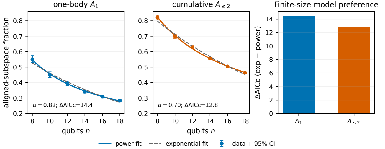
FIG. 12. Finite-size diagnostics for the half-filled U(1) family. The left panels show the full n = 8-18 overlap data together with the fitted power and exponential models; the right panel summarizes the model-selection difference \Delta AICc = AICc_{exp} - AICc_{power} . Positive values favor the power model within the tested finite-size window only.
