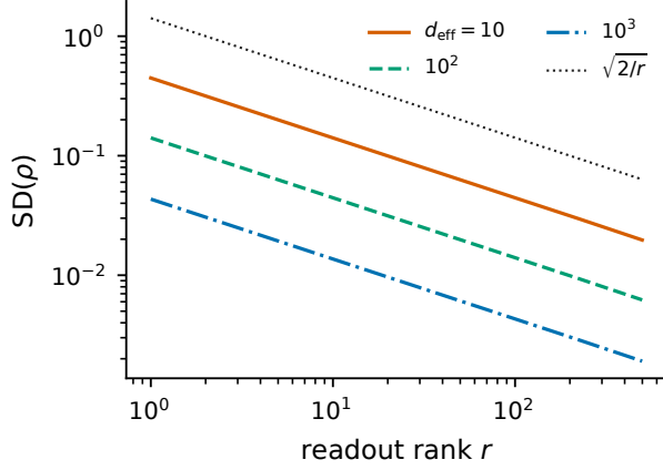
FIG. 8. Exact random-orientation fluctuation scale for representative effective dimensions. The standard deviation of \rho narrows with increasing readout rank and effective spectral dimension; this is compatible with a strongly anisotropic covariance whenever rd_{\text{eff}} is large.
