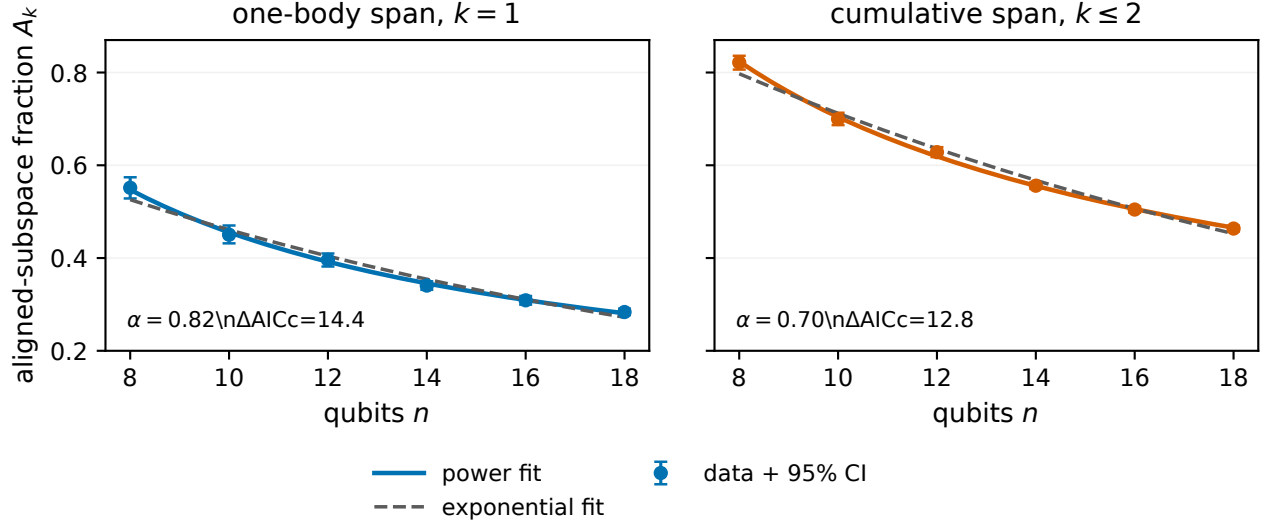
FIG. 6. Finite-size low-weight alignment in the half-filled U(1) family. Points and error bars are circuit-level means and 95% bootstrap intervals for the cross-fitted leading rank- r_1 tangent subspace. Solid curves are the two-parameter power fits and dashed curves are exponential fits over n = 8 –18. Positive \Delta \text{AICc} favors the power model over the tested window. The comparison is descriptive finite-size model selection, not an asymptotic or hydrodynamic theorem.
