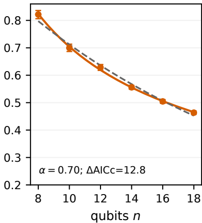
cumulative A_{\leq 2}
