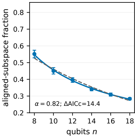
one-body A_1
