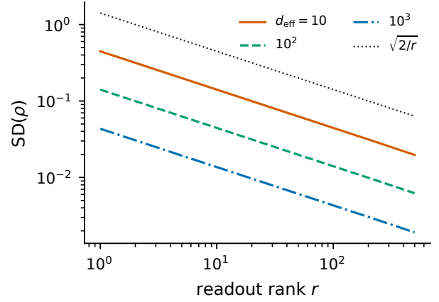
FIG. 9. Exact random-orientation fluctuation scale for representative effective dimensions. The standard deviation of \rho narrows with increasing readout rank and effective spectral dimension; this is compatible with a strongly anisotropic covariance whenever rd_{\text{eff}} is large.
