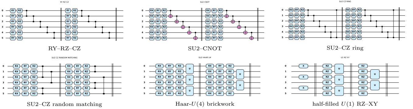
FIG. 13. Individual PennyLane circuit schematics used by the numerical campaign. Gate parameters are hidden in the drawings, while the source constructors and complete numerical profiles are archived with the code and results.
