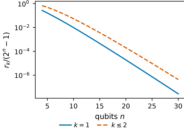
FIG. 9. Rank fractions for low-weight diagonal readouts under full computational-basis support. Polynomially growing low-weight spaces occupy an exponentially shrinking fraction of the centered record.
