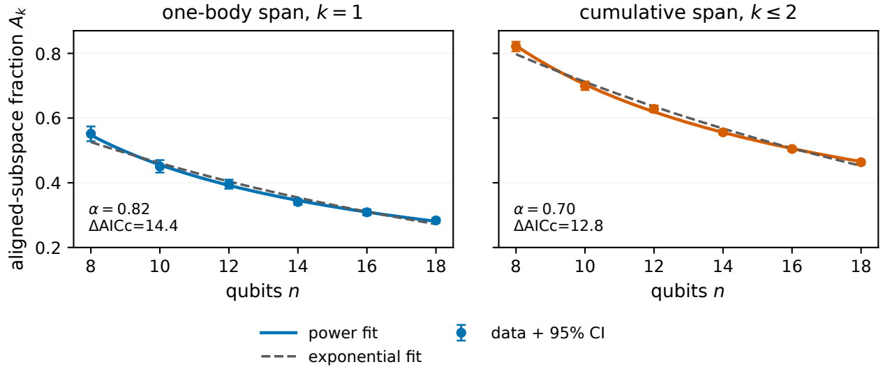
FIG. 7. Finite-size low-weight alignment in the half-filled U(1) family. Points and error bars are circuit-level means and 95% bootstrap intervals for the cross-fitted leading rank- r_1 tangent subspace. Solid curves are the two-parameter power fits and dashed curves are exponential fits over n = 8 –18. Positive \Delta\text{AICc} favors the power model over the tested window. The comparison is descriptive finite-size model selection, not an asymptotic or hydrodynamic theorem.
