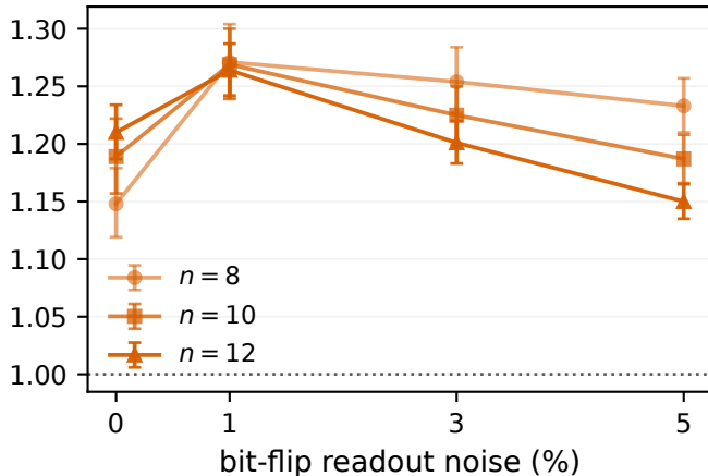
U(1)
