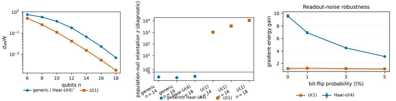
FIG. 11. Supporting diagnostics. Left: effective spectral fraction d_{\text{eff}}/N . Center: population-null orientation diagnostic for representative generic/Haar and U(1) points. Right: aligned-to-physical directional gradient-energy gain under readout bit-flip noise. The noise comparison re-estimates the aligned subspace after noise is applied and therefore does not establish robustness of a single fixed optimized observable.
