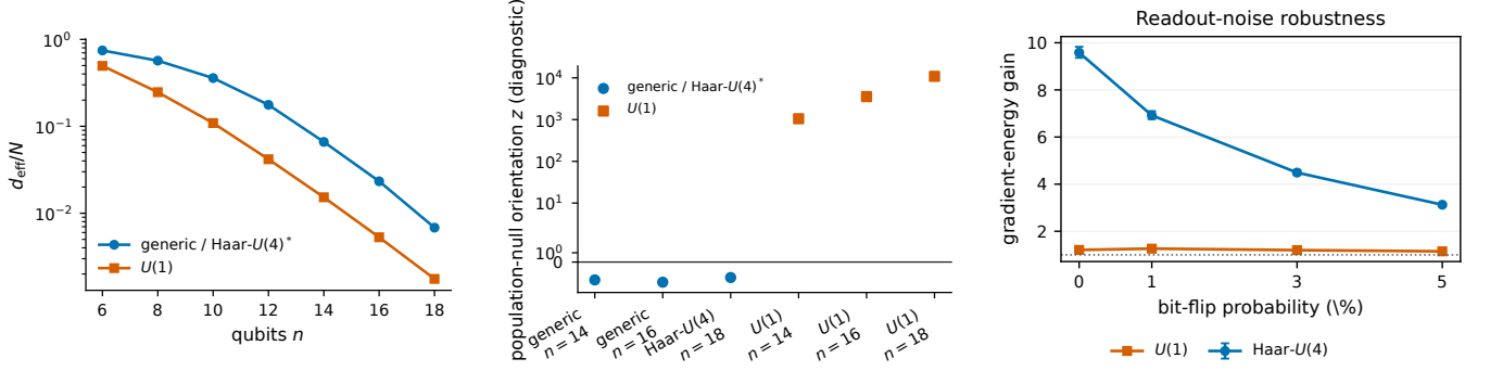
FIG. 12. Supporting diagnostics. Left: effective spectral fraction d_{\text{eff}}/N . Center: population-null orientation diagnostic for representative generic/Haar and U(1) points. Right: aligned-to-physical directional gradient-energy gain under readout bit-flip noise. The noise comparison re-estimates the aligned subspace after noise is applied and therefore does not establish robustness of a single fixed optimized observable.
