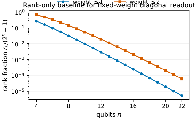
FIG. 2. Rank-only scale for fixed-weight diagonal readout under full computational-basis support. For fixed Pauli weight, the retained subspace rank grows polynomially while the centered score-space dimension grows exponentially. The plotted fractions are geometric baselines only; physical retention depends on spectral orientation.
