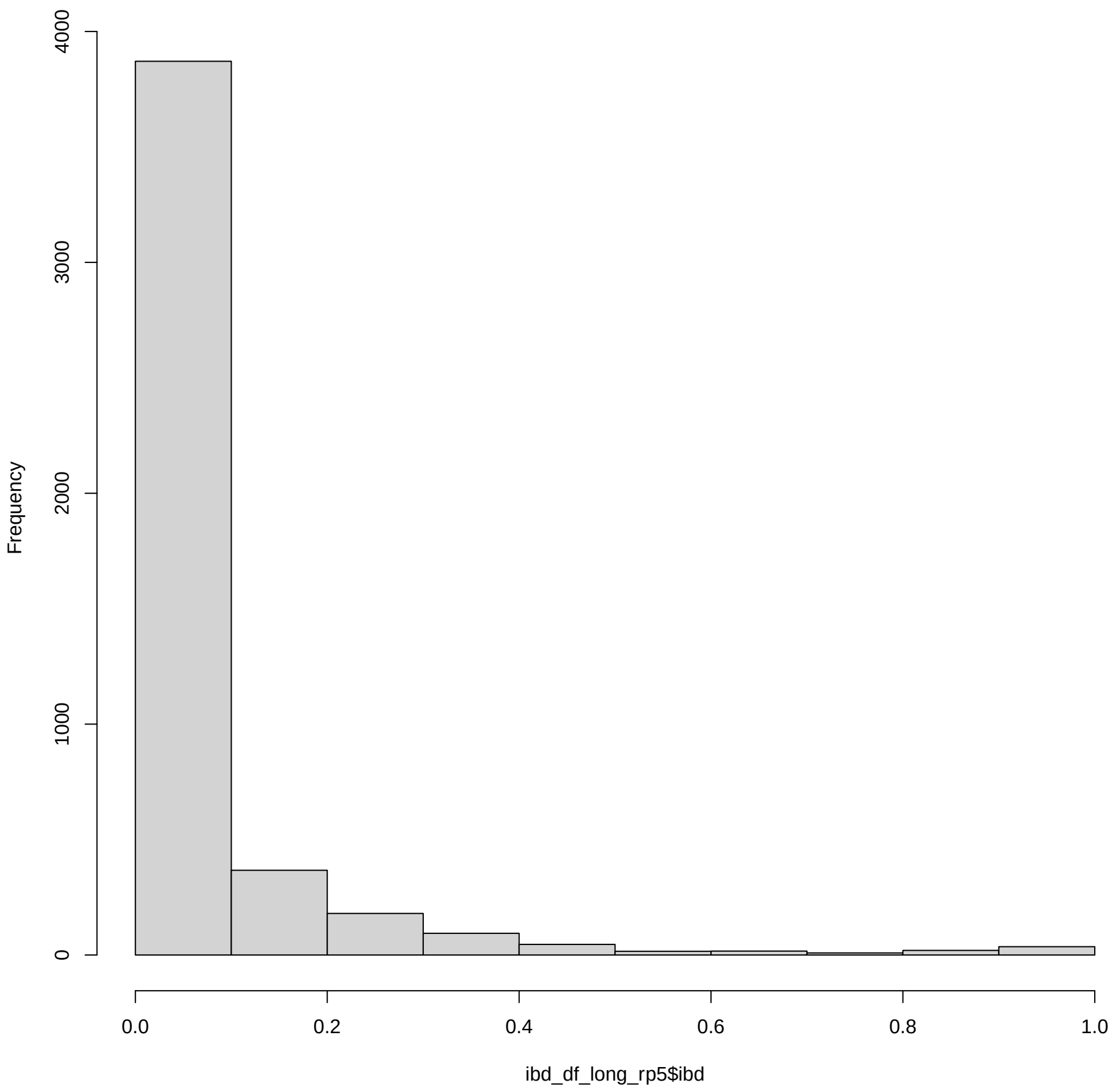
Histogram of ibd_df_long_rp5$ibd
