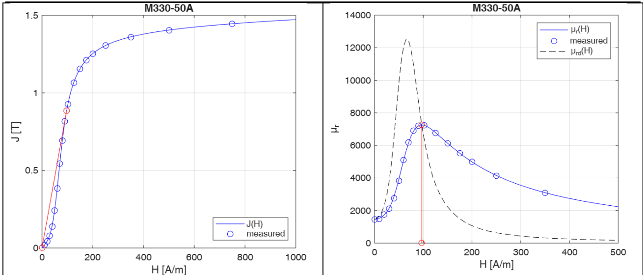
Figure 1 Magnetic characteristic (left) J(H) and (right) relative permeability and differential relative permeability
