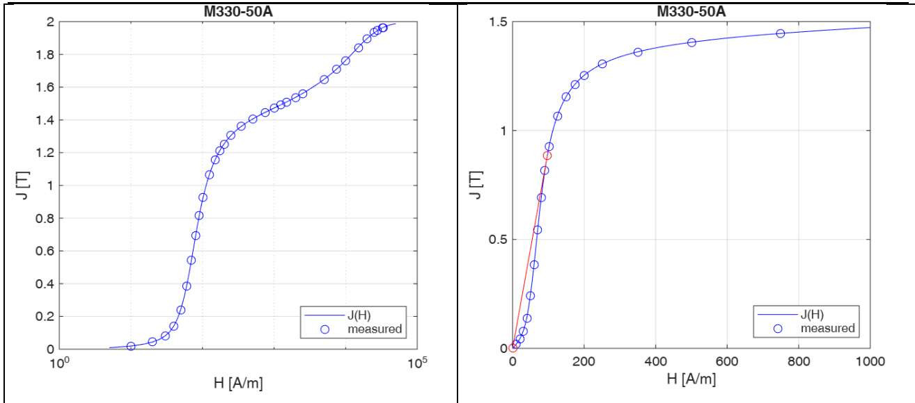
Figure 2 Polarization J(H) for the whole measured range and for the region of low field strength
