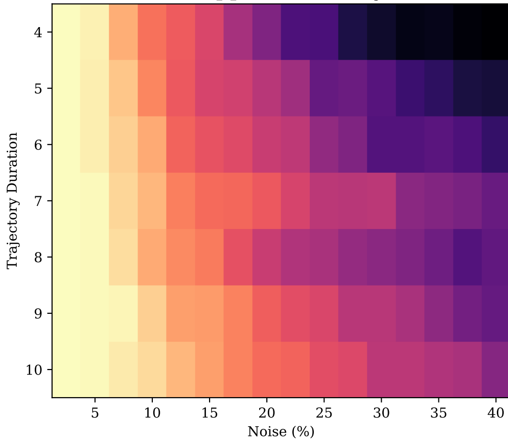
Exact Support Recovery Rate
