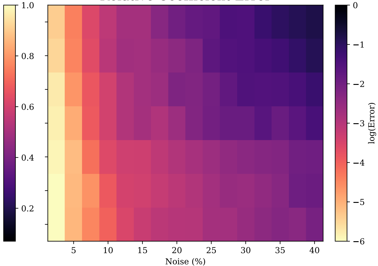
Relative Coefficient Error
