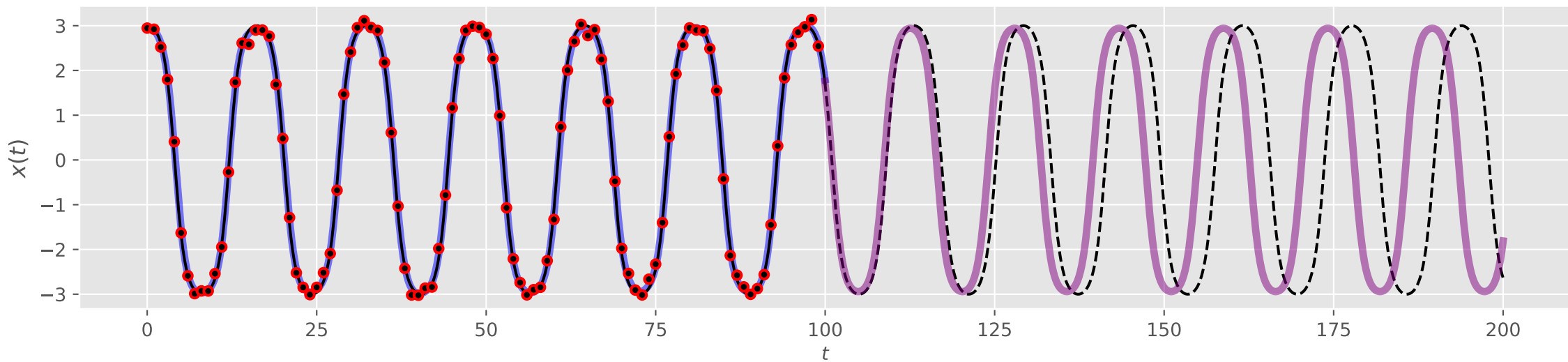
Cubic Model
