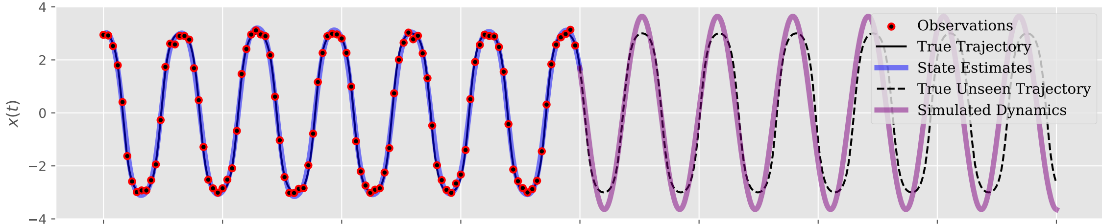
Cubic Model
