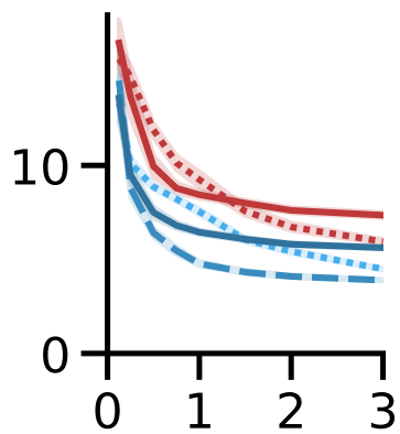
dconvert
