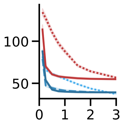
x265
