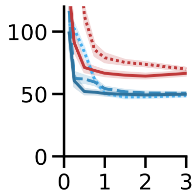
x264
