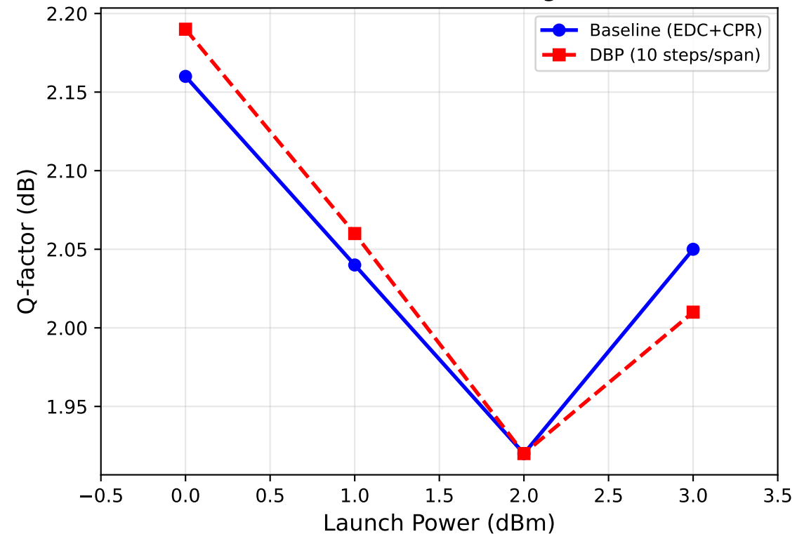
MVB-5 (1600km, 16QAM, Long Distance)
