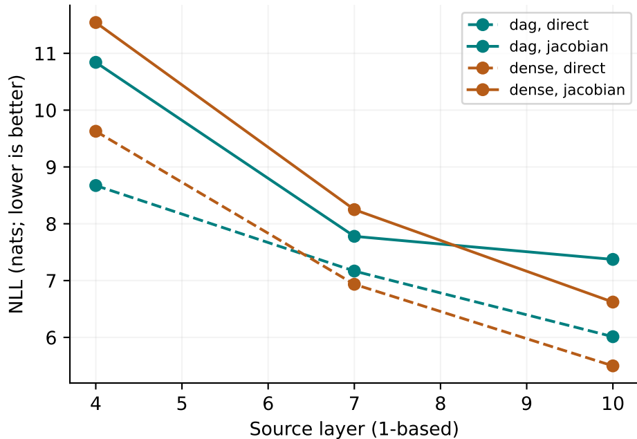
Natural next-token readout
