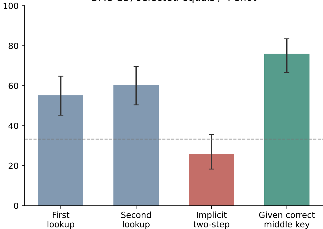
DAG 1B, selected equals / 4-shot
