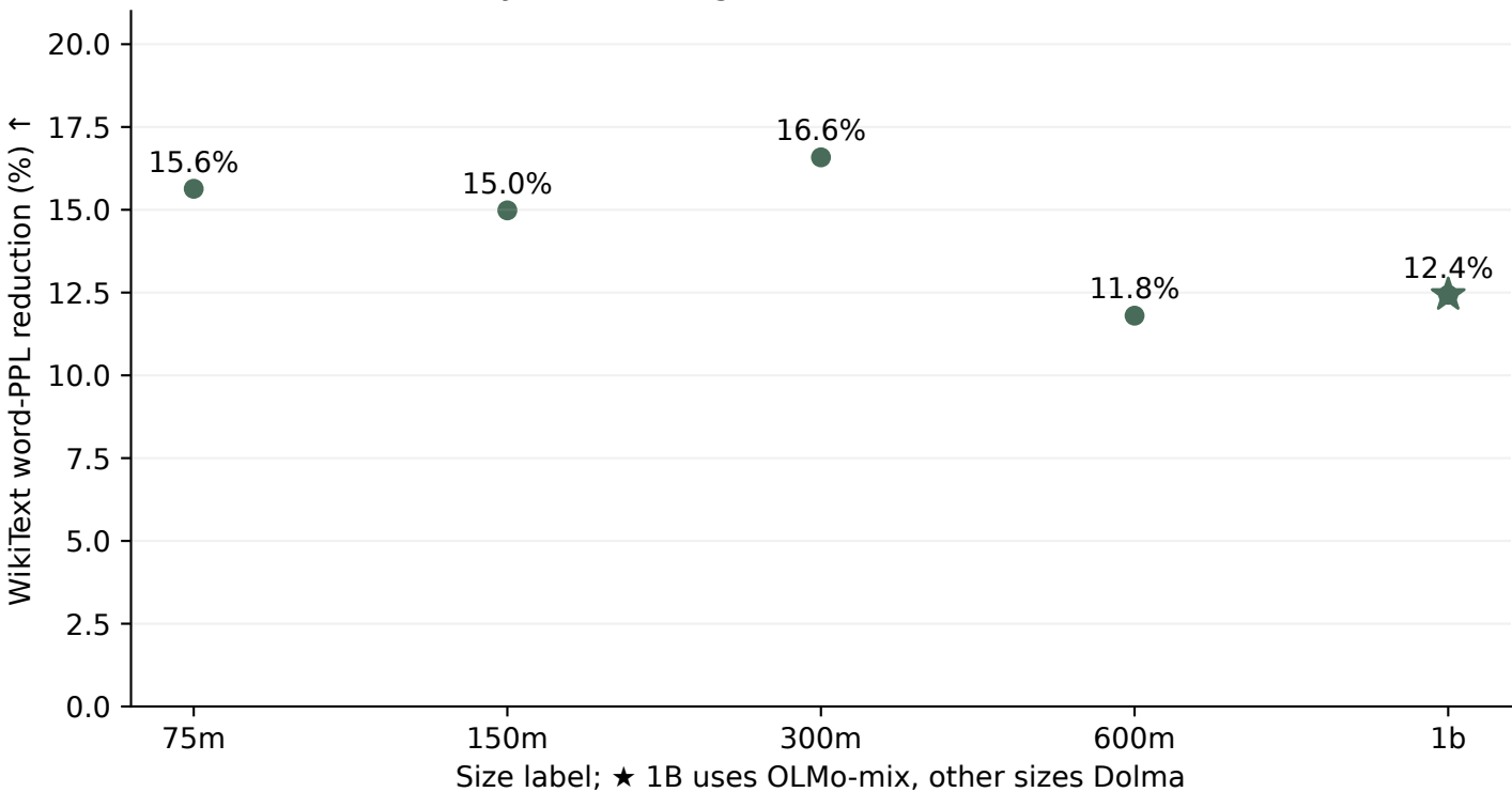
FourWay's WikiText gains remain across tested sizes
