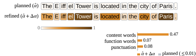
(b) The graph changes token by token
