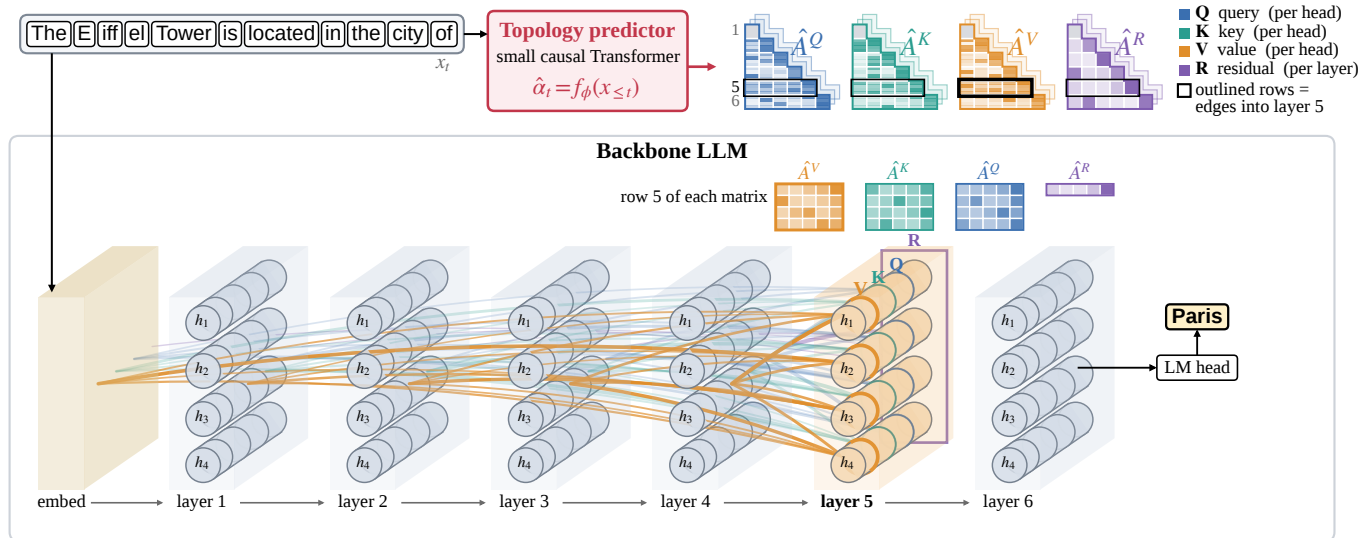
(b) The graph changes token by token
