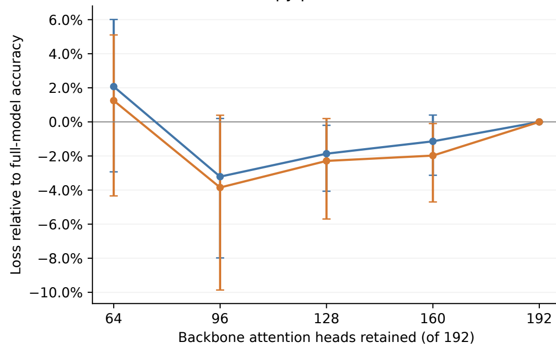
WikiText sampled positions
