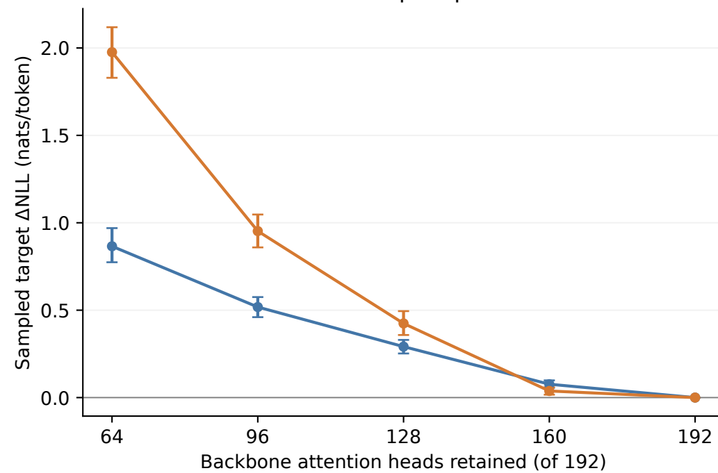
WikiText sampled positions
