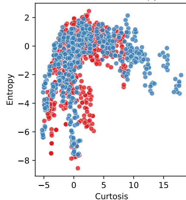
Kurtosis vs Entropy
