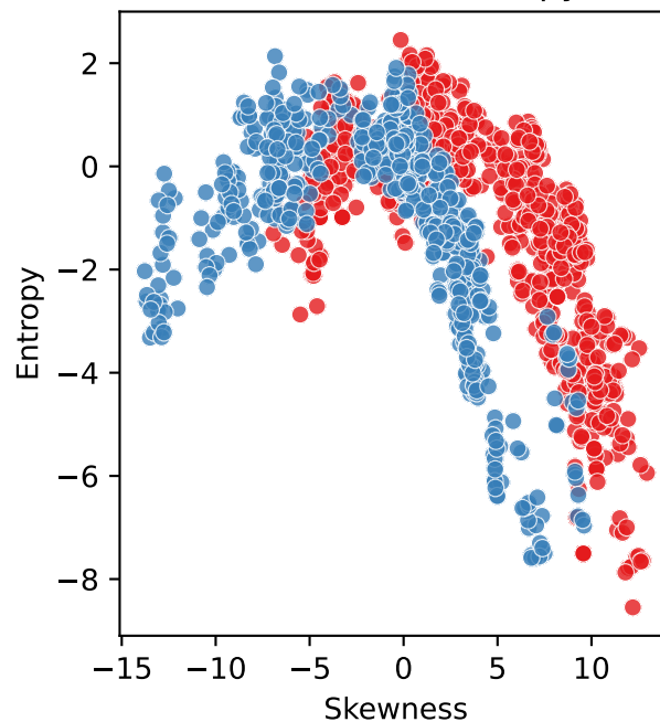
Skewness vs Entropy
