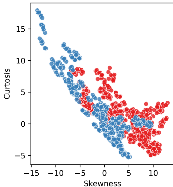
Skewness vs Kurtosis
