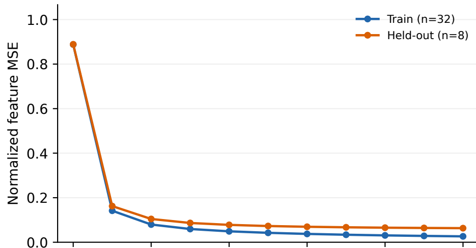
A Caption-content MSE — training objective
