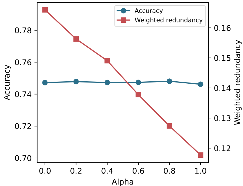
Wine
