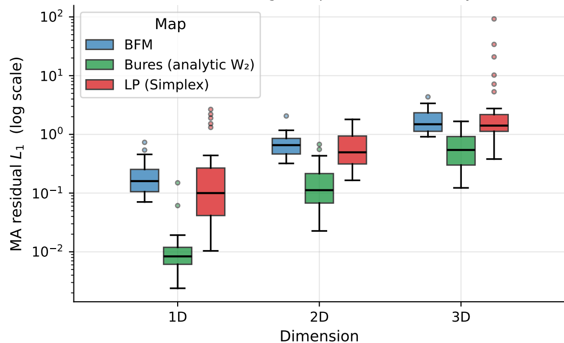
BFM vs Bures vs LP: Monge-Ampère residual ( L_1 ) by dimension
