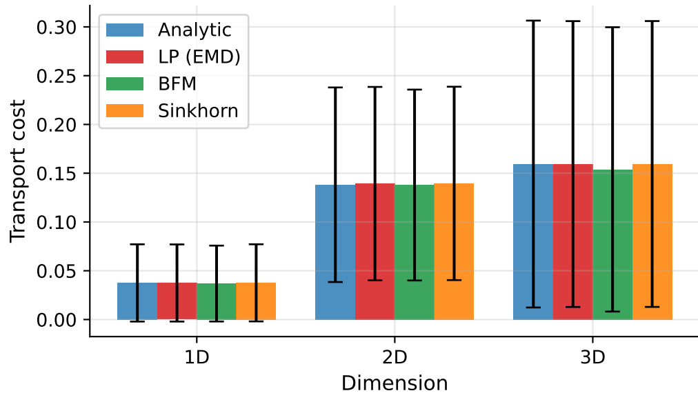
(A) Transport cost — mean \pm std
