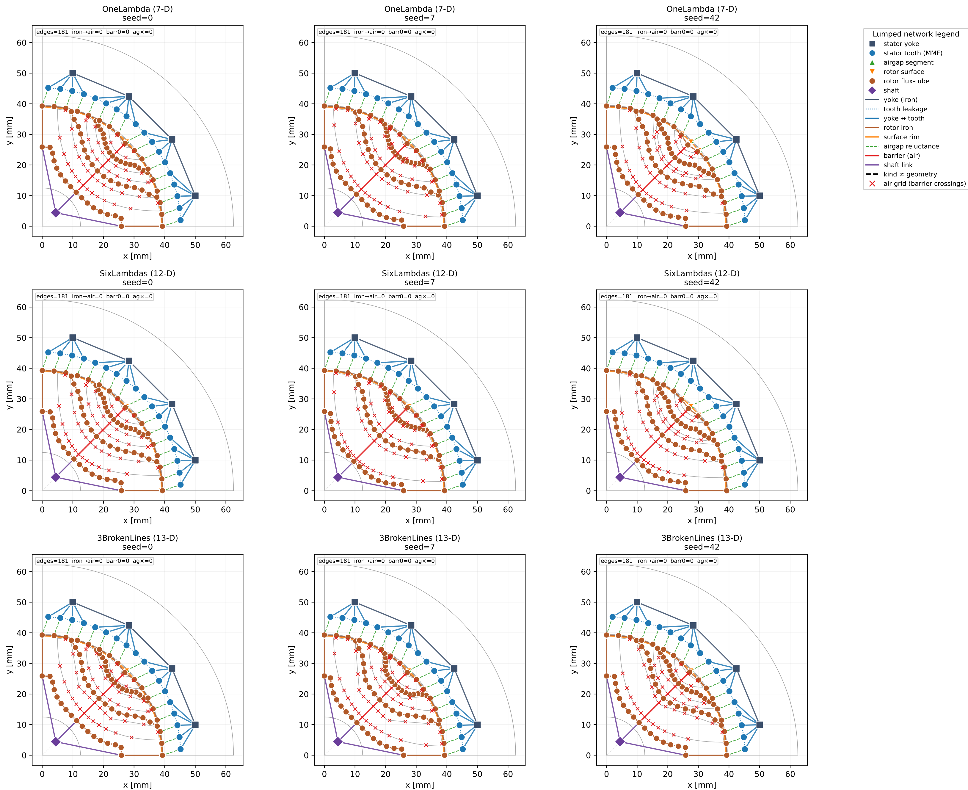
Lumped reluctance network — FINE granularity rows: barrier parameterisation, columns: random parameter sample
