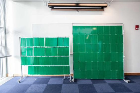
(a) RFocus 1-bit RIS原型
