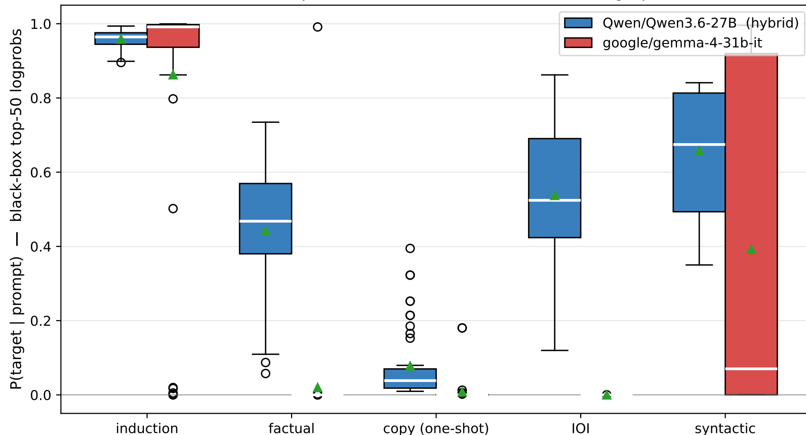
H31 — same probes, different vendor behavioral fingerprint
