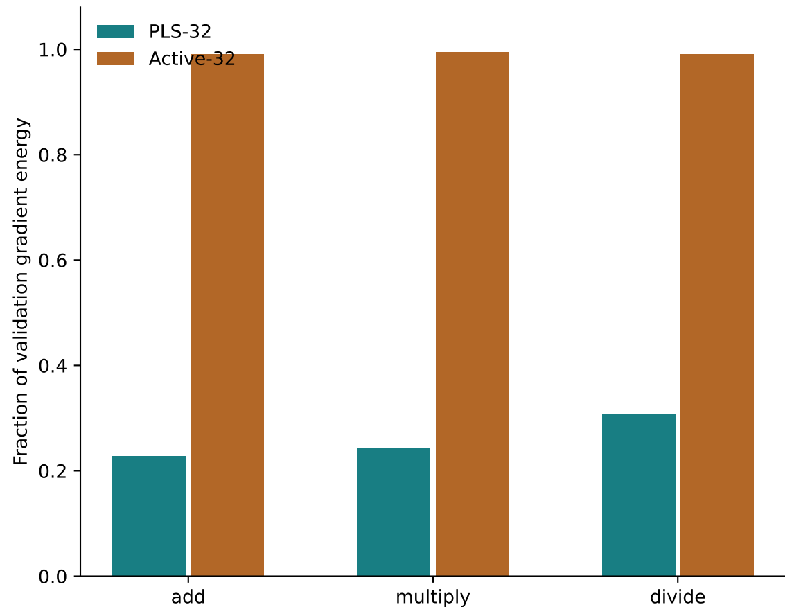
Coordinates retain different local sensitivities (1.7B)
