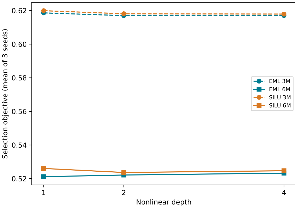
Depth at matched coefficient budgets
