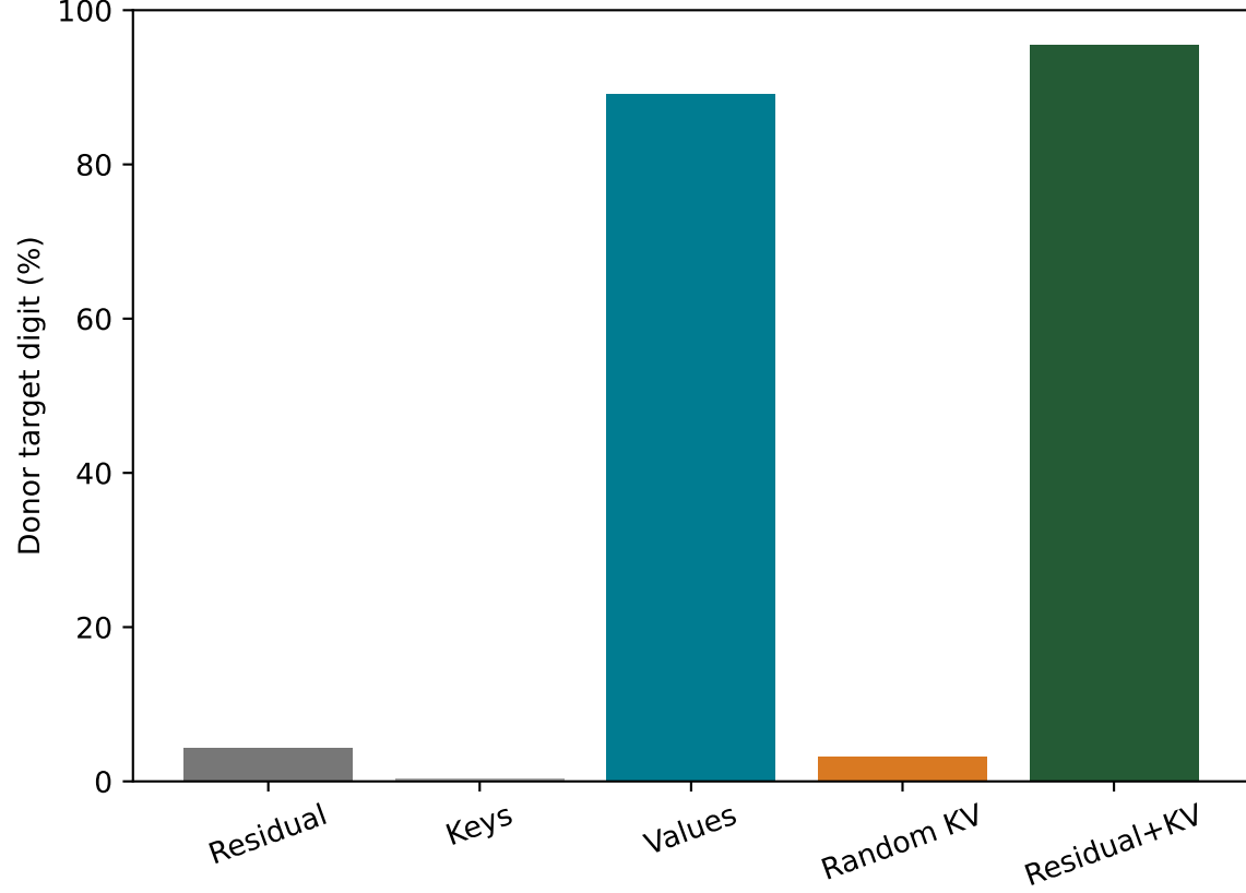
Original-model causal interventions
