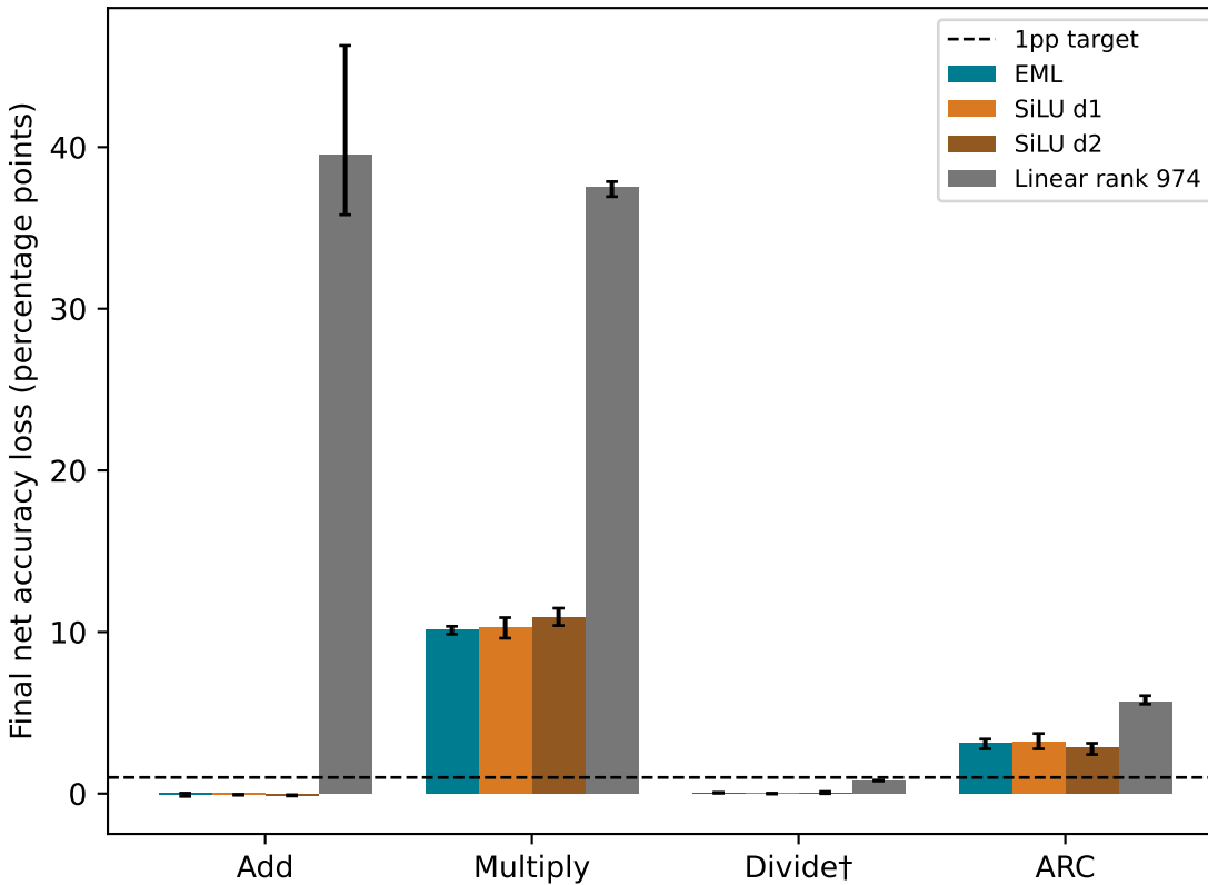
Complete MLP replacement
