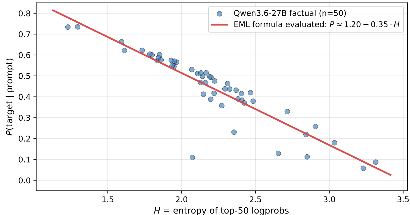
Black-box derivation on Qwen3.6-27B factual recall
