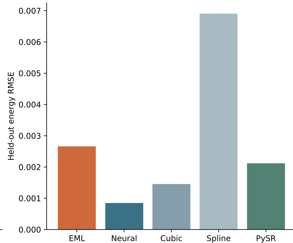
Pendulum: accurate within range
