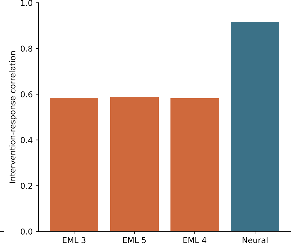
LLM: causal fidelity remains limited
