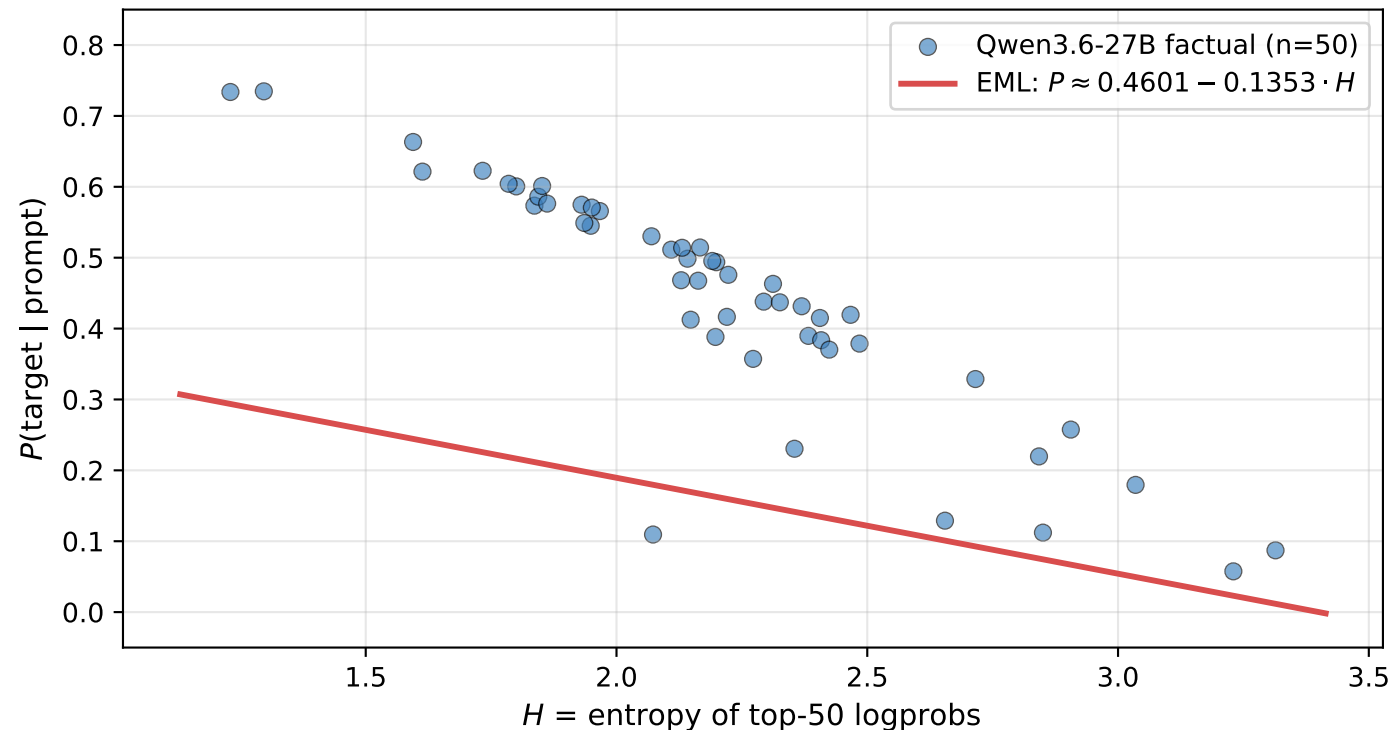
H31 — black-box derivation on Qwen3.6-27B factual recall
