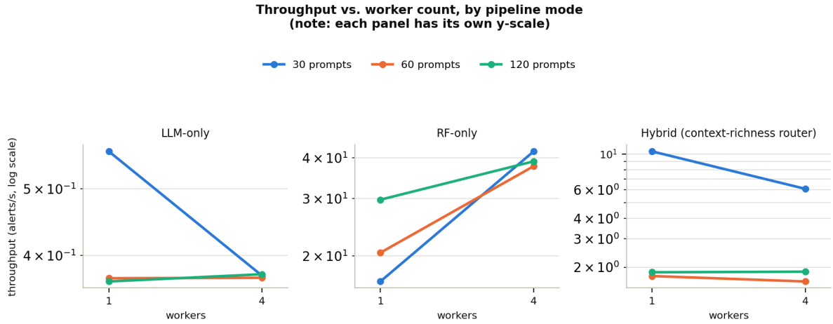
Fig. 3 Throughput vs. worker count, faceted by pipeline mode (note each panel has its own log-scale y-axis — the three modes differ by roughly two orders of magnitude and are not comparable on a shared axis). RF-only throughput scales with worker count as expected for local CPU-bound inference; LLM-only and hybrid do not, because Groq’s per-minute token budget is shared across worker threads regardless of concurrency. Generated by docs/paper/figures/generate_figures.py directly from week7_scalability_benchmark.json (PROGRESS.md item T2c).
