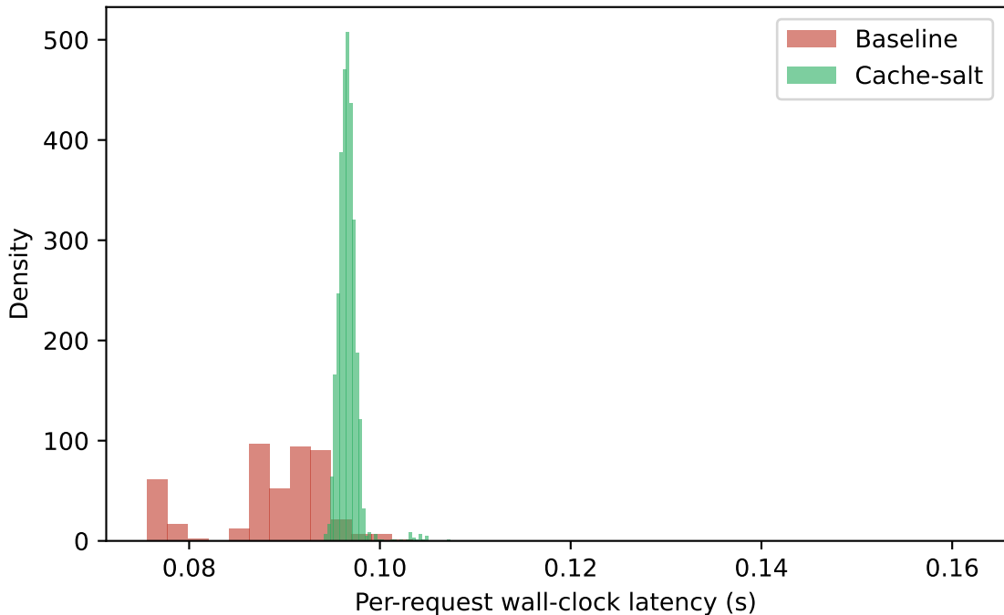
Per-request latency distribution, baseline vs. salted
