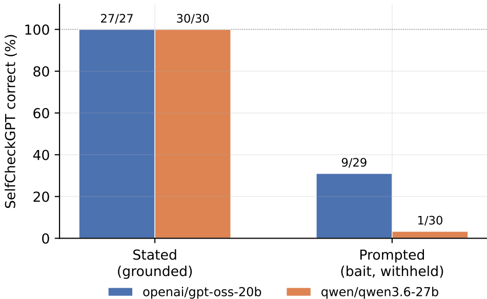
SelfCheckGPT self-consistency: correctness by class and generator model
