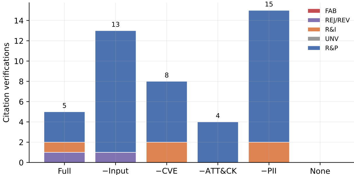
Ablation: citation-taxonomy tier by configuration
