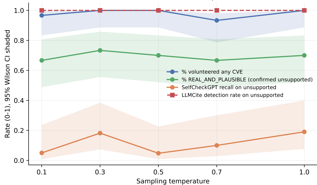
Temperature sensitivity: citation volunteering and detection (30 withheld-CVE alerts, 3 resamples each)
