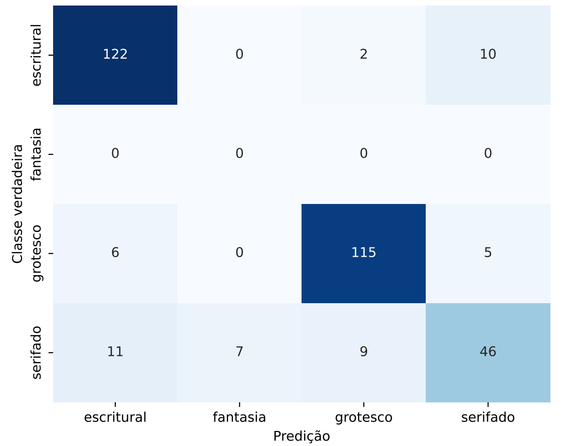
5. EfficientNet (Base)
