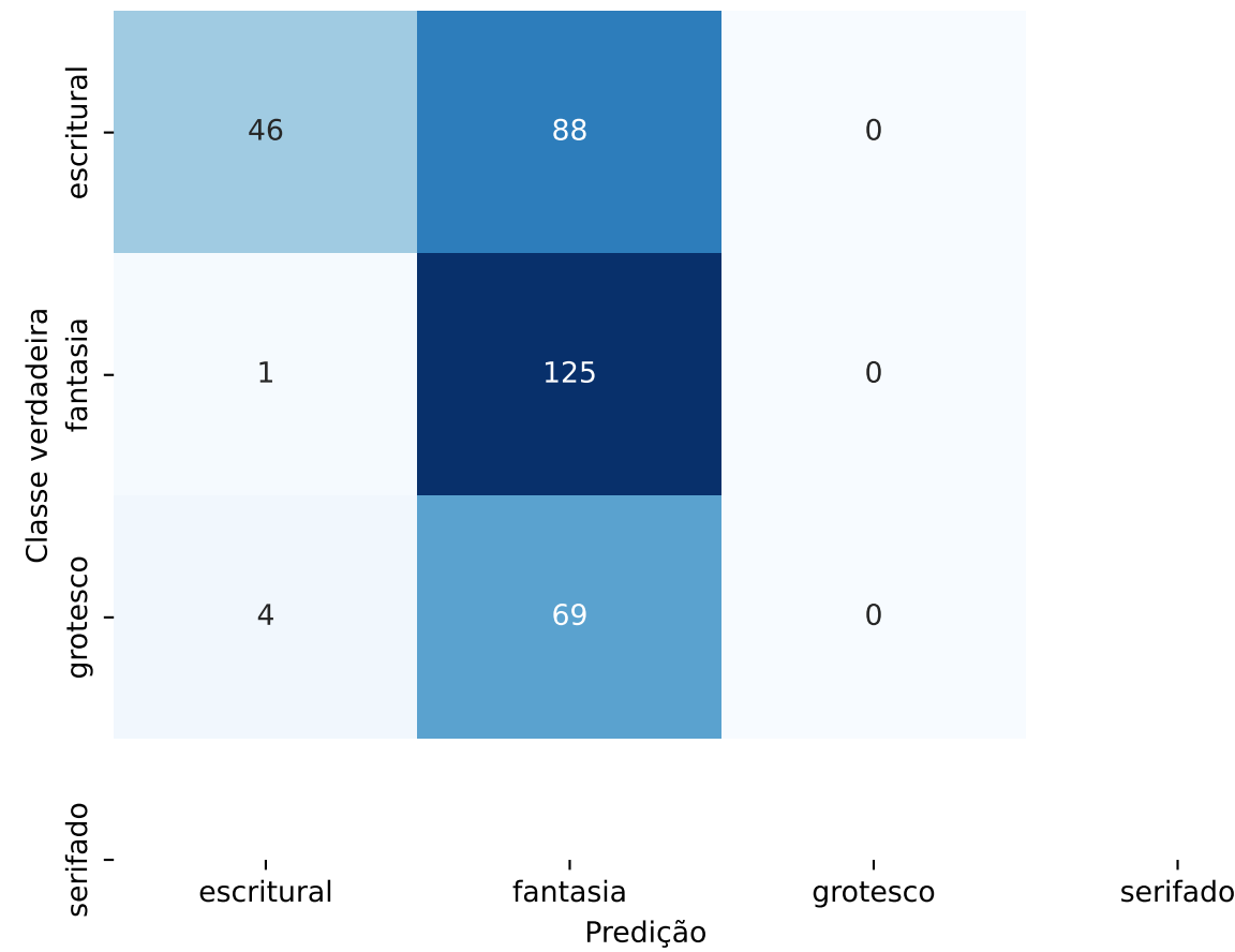
5. EfficientNet (Base)
