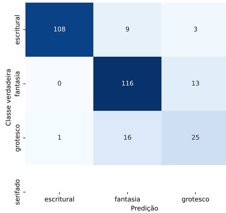
5. EfficientNet (Base)
