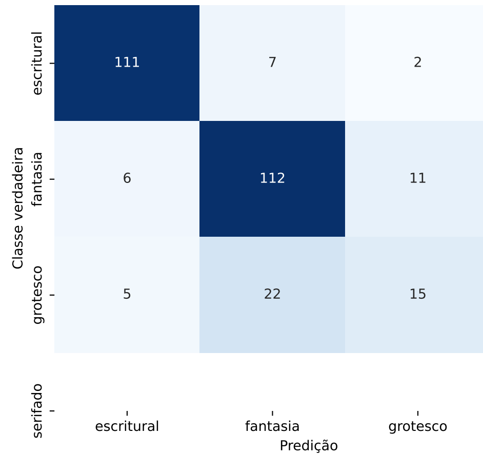
5. EfficientNet (Base)
