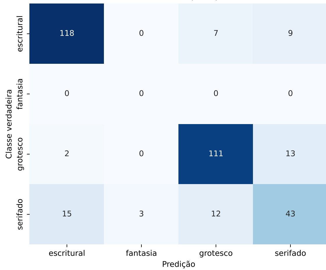
ResNet-18 (Final)
