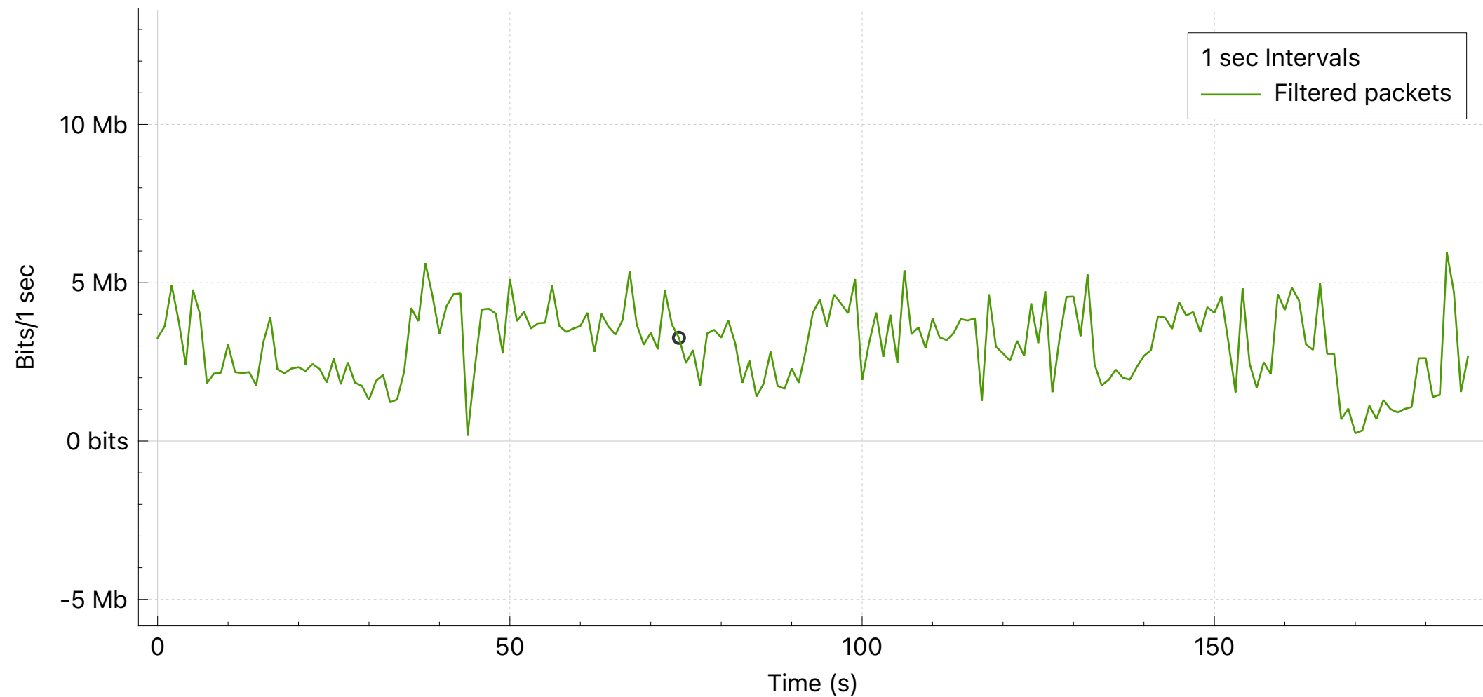
Wireshark I/O Graphs: RB_Display_P2S_test_Messenger_Call.pcapng
