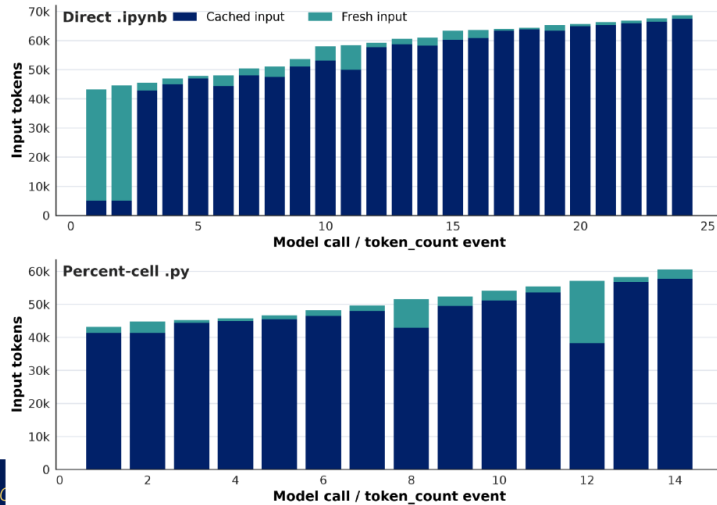
Fig. 6: The notebook workflow took more model calls. Each call is another chance for context, tool output, and file state to enter the next step.
