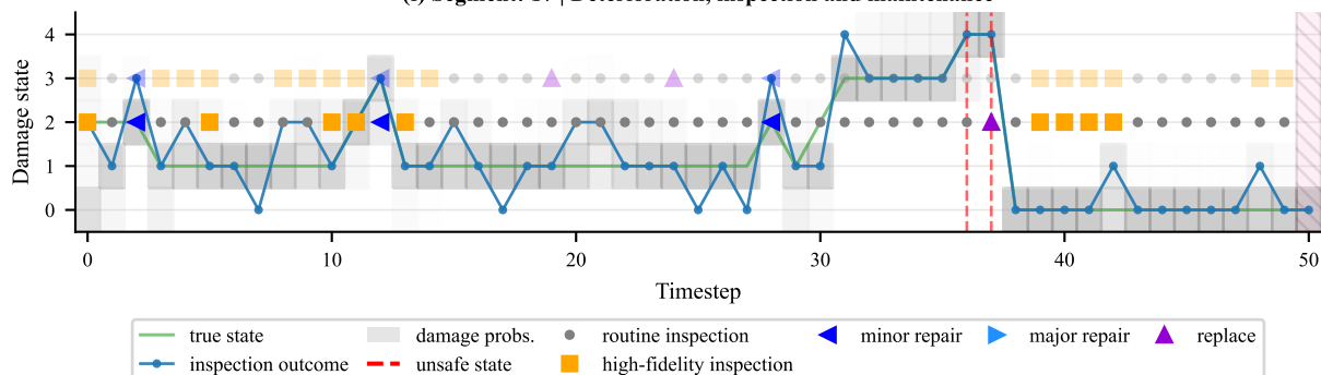
(f) Segment: 17 | Deterioration, inspection and maintenance
