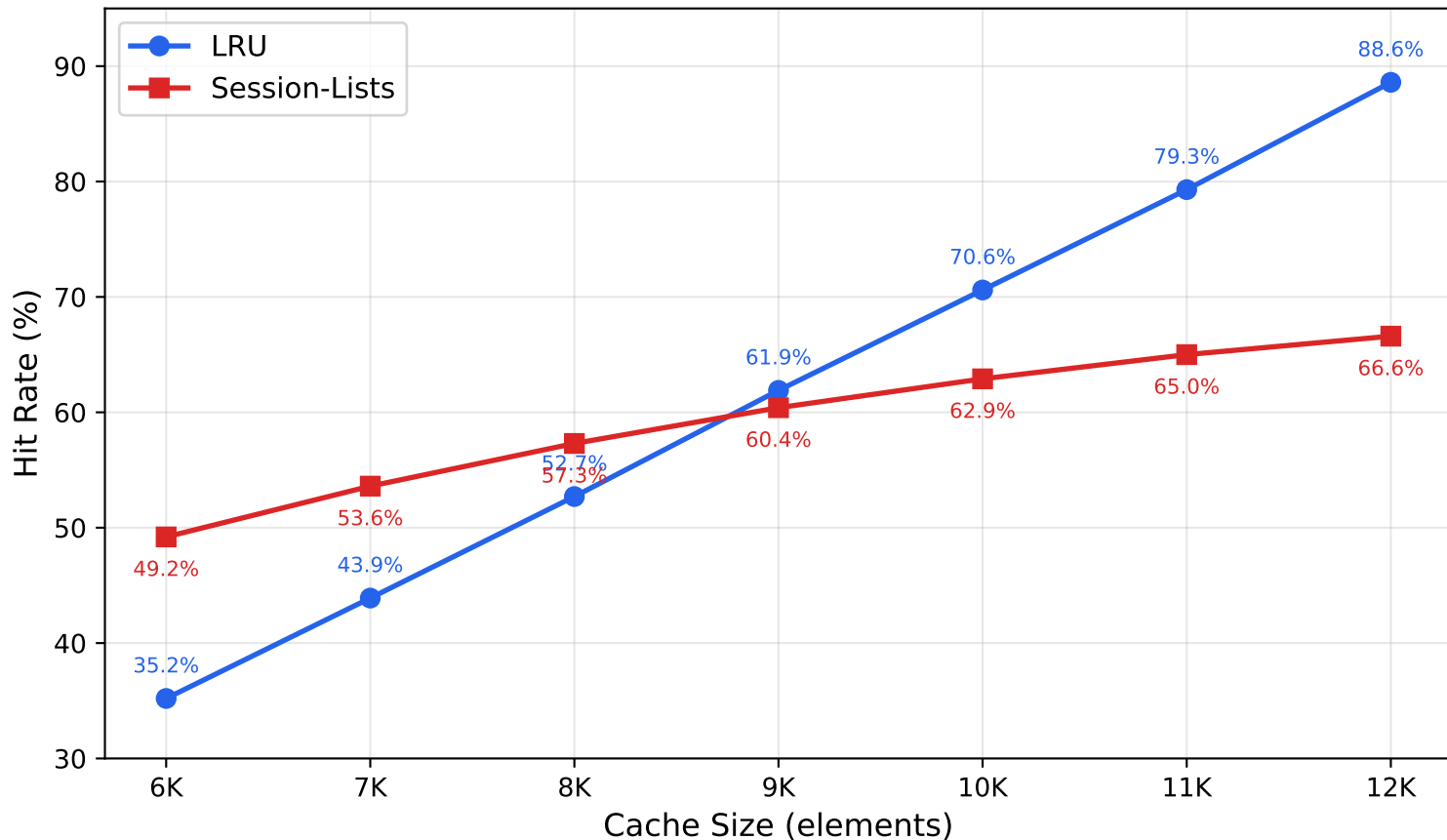
Hit Rate vs Cache Size — Weka Trace (50 conversations)
