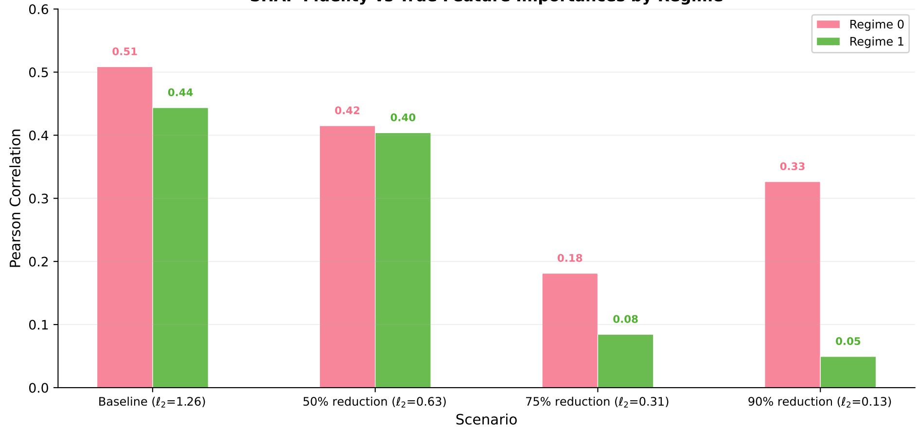
SHAP Fidelity vs True Feature Importances by Regime
