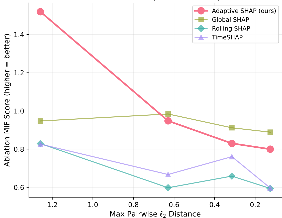
Ablation: Most Important First (p50)
