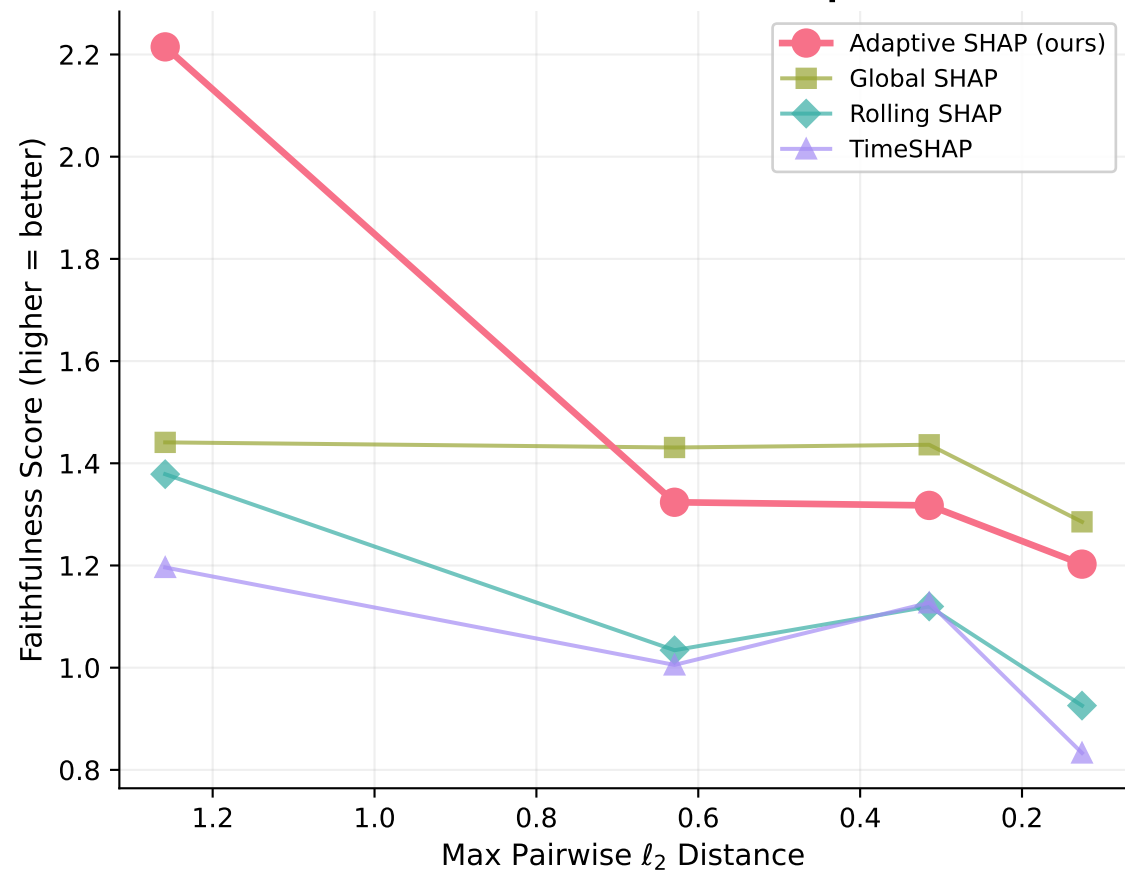
Faithfulness (Perturbation p50)
