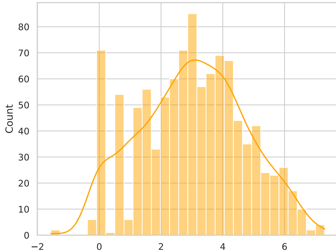
Box-Cox Transformed Data Distribution ( \lambda=0.04 )
