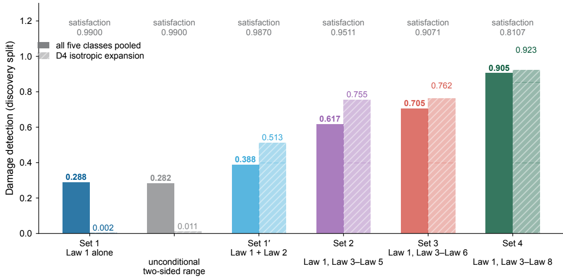
Fig. S10 PRIS law sets and an unconditional two-sided contact band. Discovery-split criteria are arranged from Law 1 through the successive PRIS law sets. The unconditional two-sided range is included as a comparator. Solid bars show pooled detection across perturbation classes, whereas hatched bars isolate isotropic expansion. Colours identify the criteria. Text above each group gives experimental-structure satisfaction.
