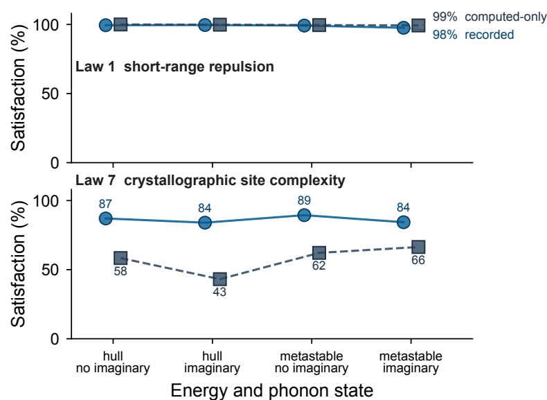
Fig. S22 PRIS satisfaction across energy, phonon and experimental-record classes. The horizontal axis crosses on-hull or metastable status with the absence or presence of imaginary phonon modes. The upper and lower profiles show satisfaction of Law 1 and Law 7, respectively. Solid blue circles denote experimentally recorded structures, and dashed grey squares denote computed-only structures. Connecting lines guide the eye.
